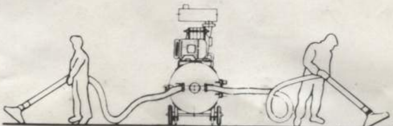
The textrim is being used as a mobile machine for two point simultaneous suction cleaning duty.
